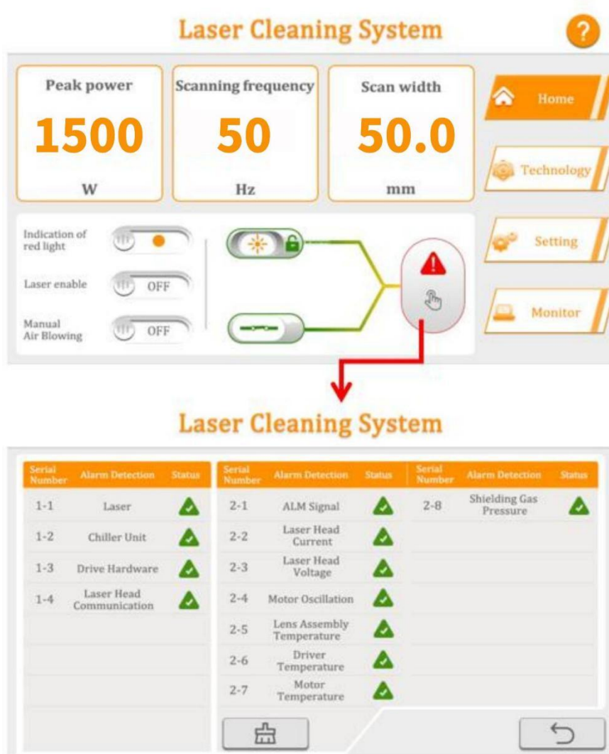
Figure 4.7 Alarm Page
