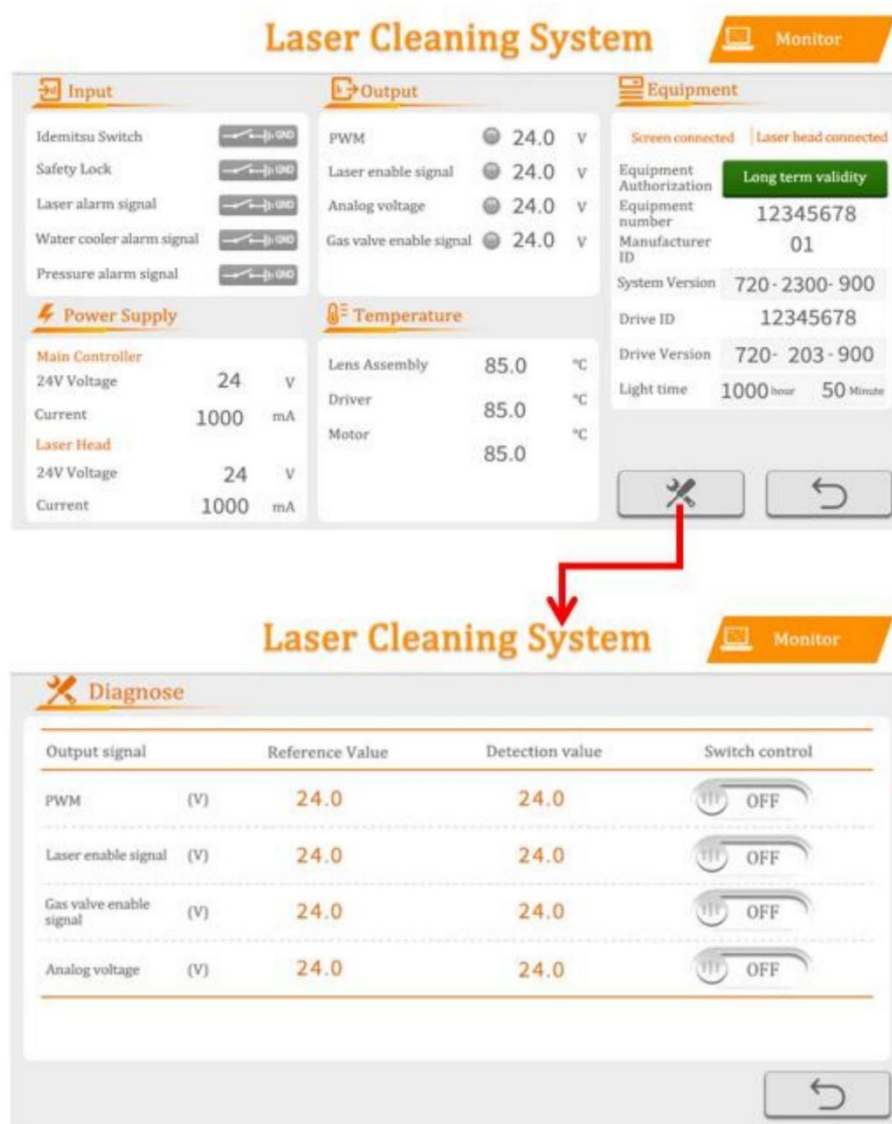
Figure 5.6 Diagnostic Page
